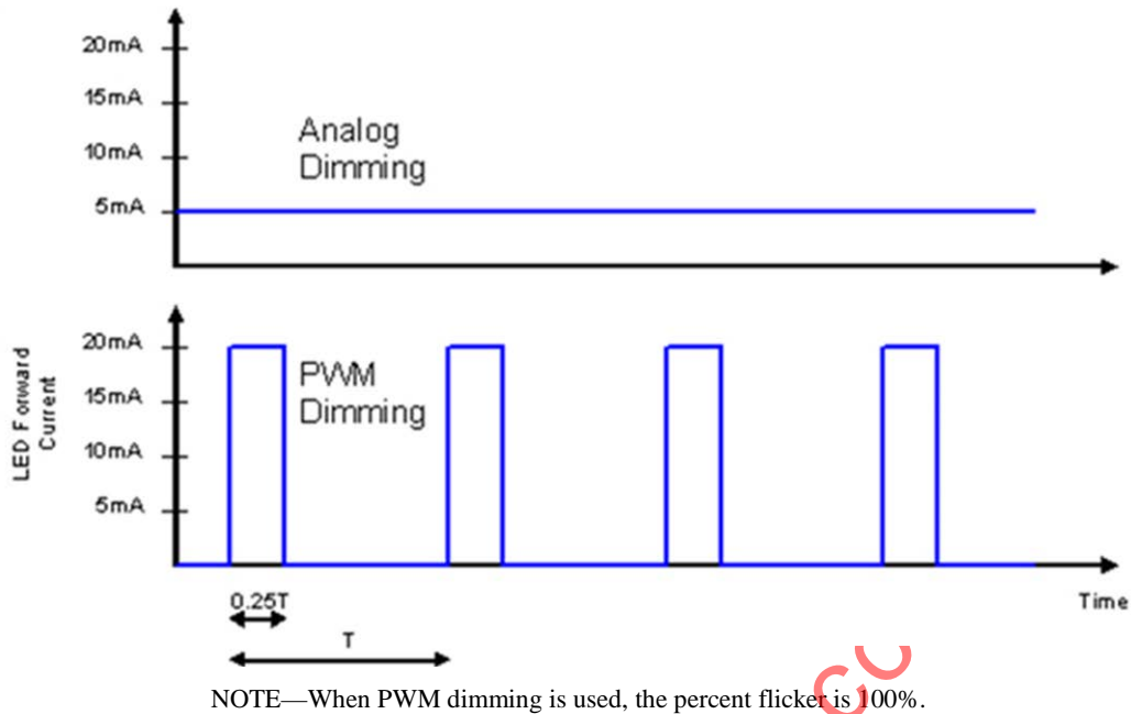
Figure 11—Analog and PWM dimming
